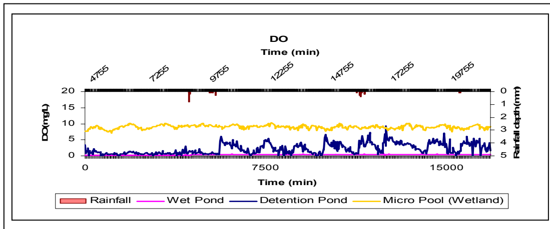
Figure 7 Value of Dissolved Oxygen at ecological pond on 11 – 23 September 2003
