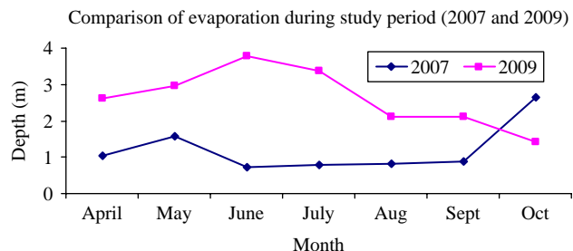
Figure 7 | Evaporation in the study area.
